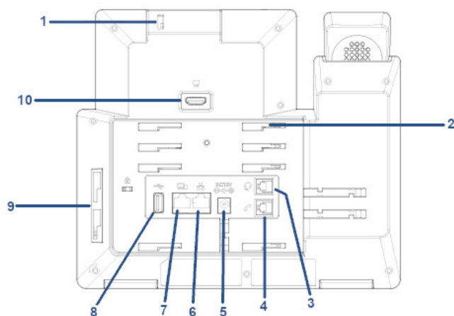
Figure 3: GXV3350 Back View
