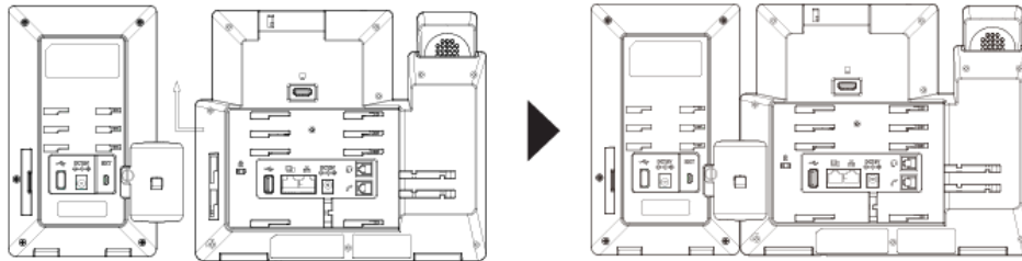
Figure 8: Connect GXV3350 and GBX20
