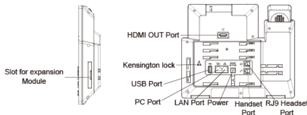
Figure 6: GXV3350 Back / Side View
