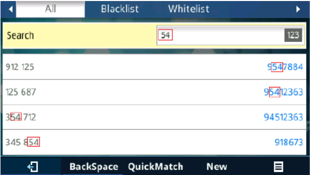
Figure 27: After Search
