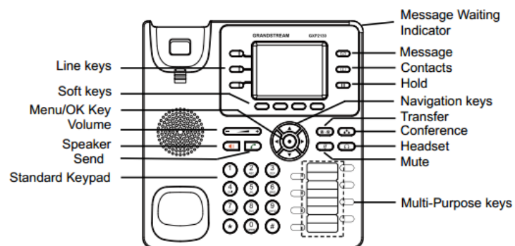
Figure 8: GXP2130 Keyboard
