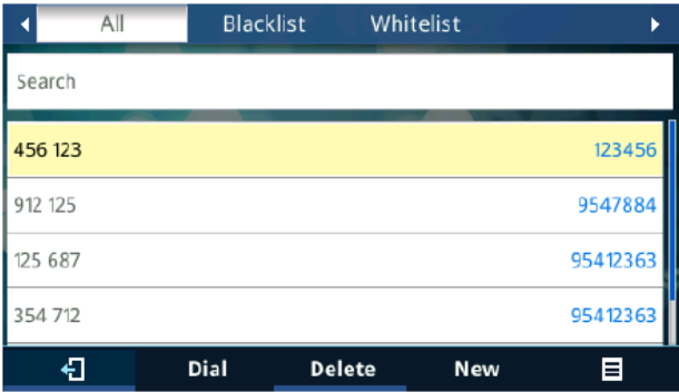
Figure 26: Before Search
