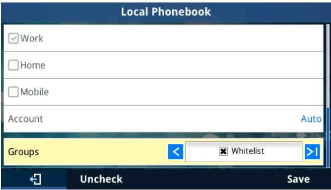
Figure 41: Black/White List
