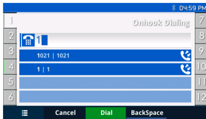
Figure 21: Predictive Dialing
