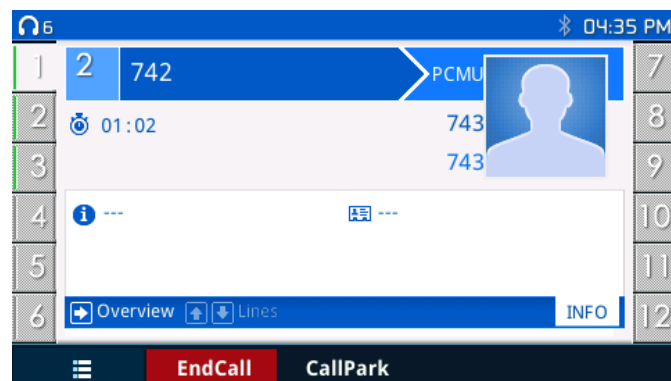
Figure 20: Making Call
