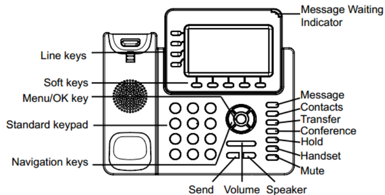
Figure 9: GXP2140 Keyboard
