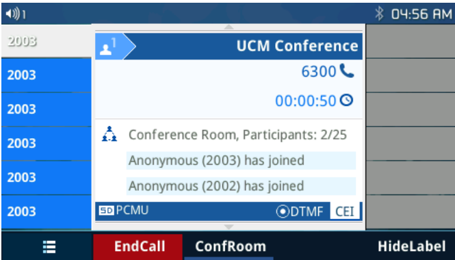
Figure 60: ConfRoom Softkey
