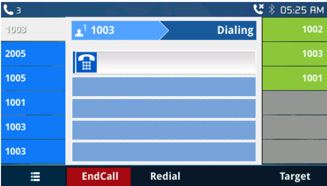
Figure 52: VPK Paging
