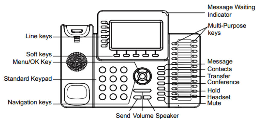
Figure 10: GXP2160 Keyboard
