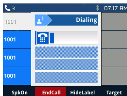
Figure 39: Group listening
