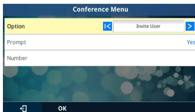
Figure 62: Conference Menu
