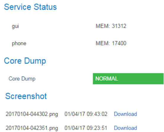
Figure 71: Screenshots
