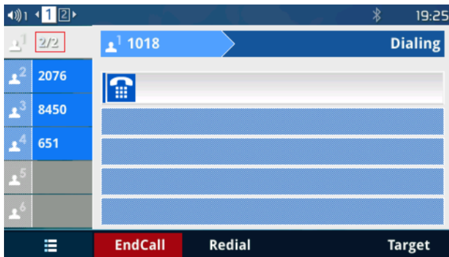
Figure 56: Account Mode
