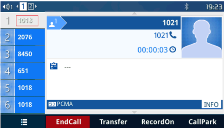
Figure 55: Line Mode
