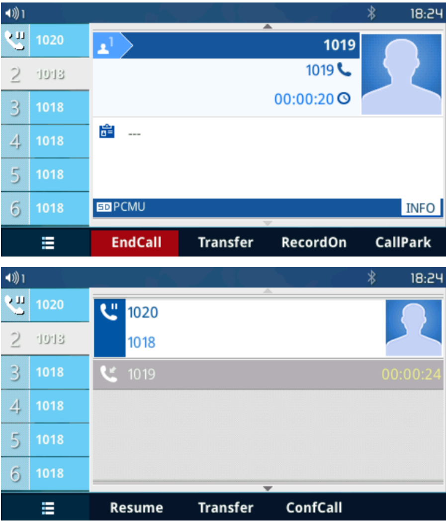
Figure 54: Line Switching
